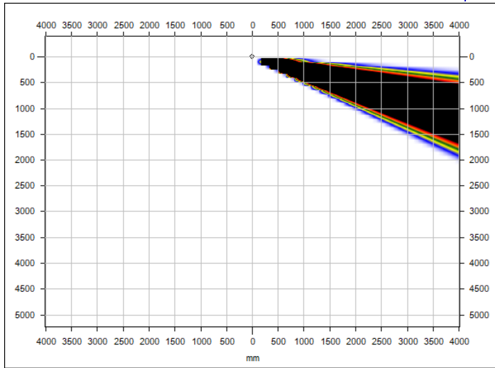
Position 1 Section 1 Mode ventilation Temperature difference 0 ° C
