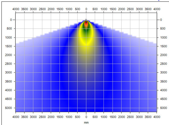
Position 4 Section 1 Mode ventilation Temperature difference 0 ° C
