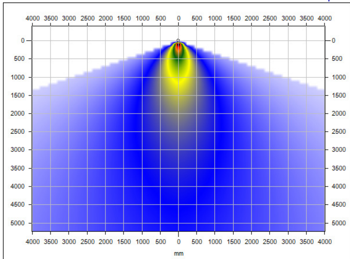
Position 2 Section 1 Mode ventilation Temperature difference 0 ° C
